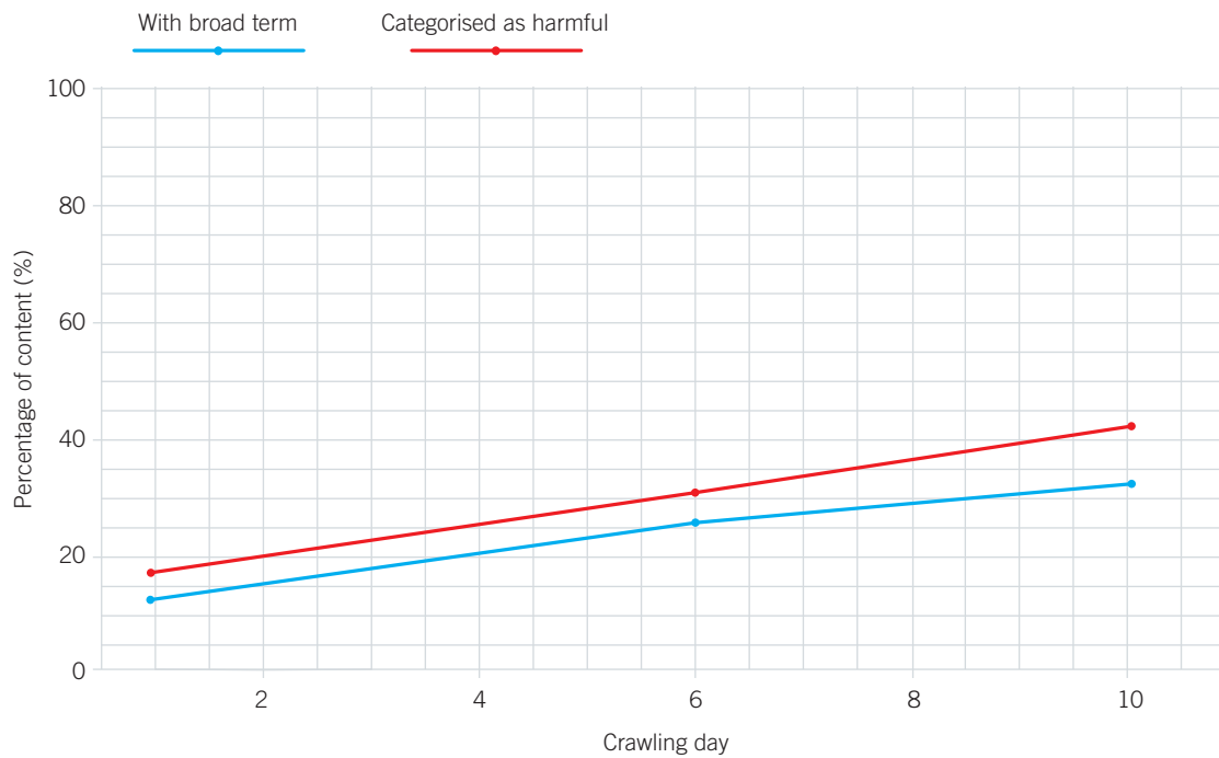
Figure 5: Progression of manually categorized content on days 1, 6 and 10 of our experiments. We map both progression of content that was classified as harmful (according to our framework) alongside progression of content whose descriptions include terms from the broad list of mental health-related terms
